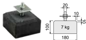
Betontegel antraciet
